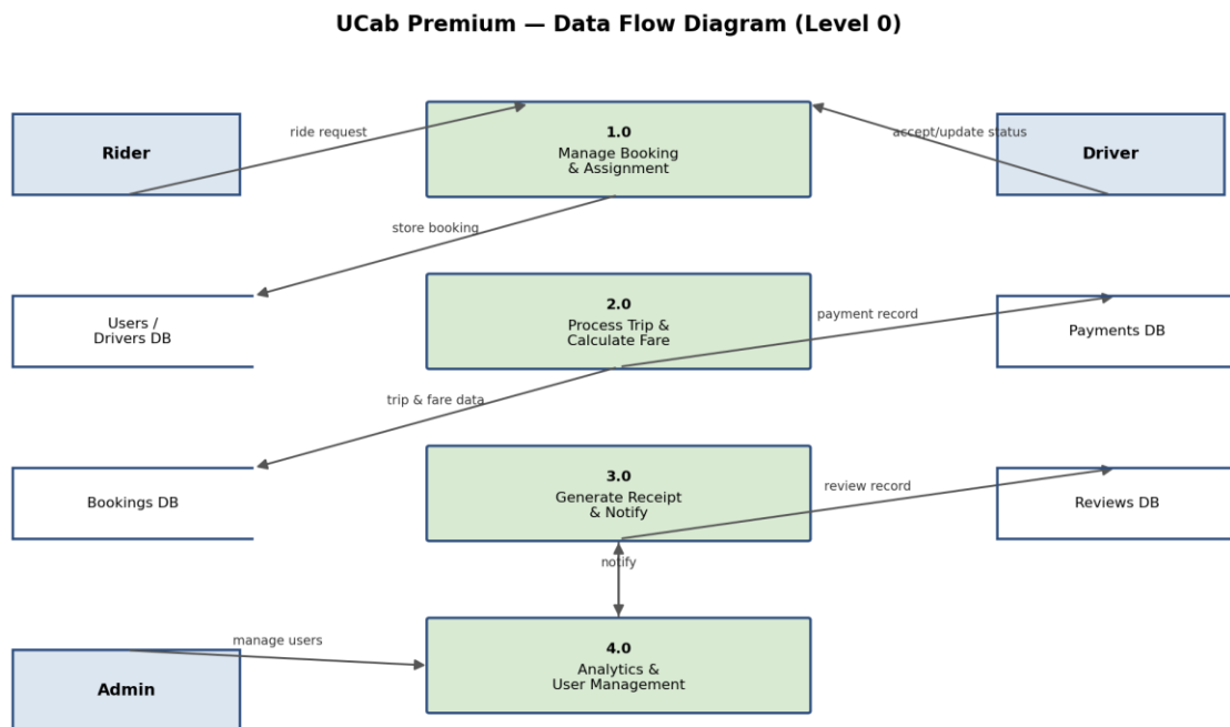
Figure 1: DFD Level 0 for UCab Premium
